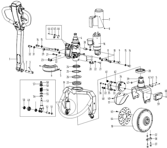
CBD12W.01-00 Steering gear assembly
